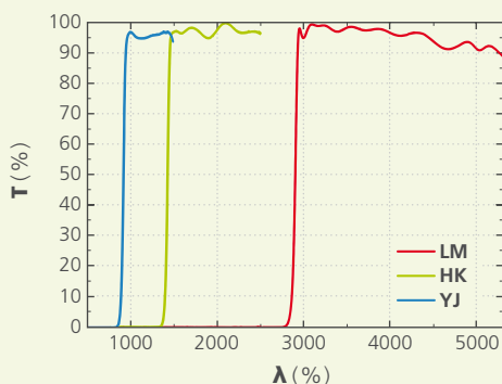
2 Transmissionsspektren der drei Filter. | Transmission spectra of all three filters.
