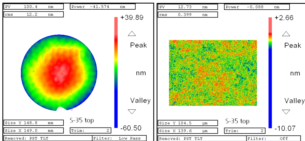
Figure 1: Surface flatness (left, \approx 100 nm PV) and roughness (right, \approx 0.4 nm RMS) of a massive SiO 2 substrate
