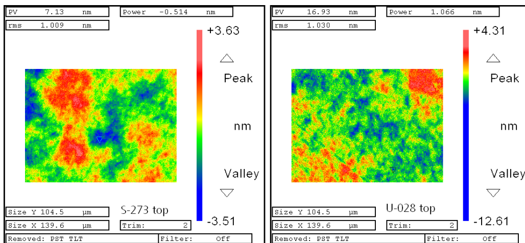
Figure 2: Surface roughnesses of a SiO 2 wafer (left, \approx 1.01 nm RMS) and an ULE wafer (right, \approx 1.03 nm RMS)
