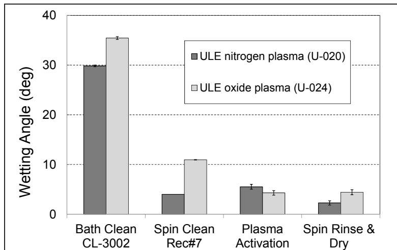
Figure 3: DI water wetting angles versus surface treatments for two ULE wafers
