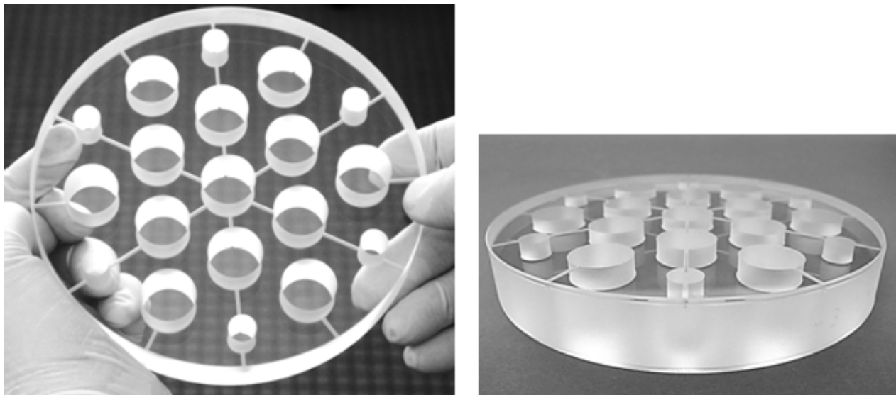
Figure 7: ULE “sandwich” structure (diameter 150 mm, thickness \approx 23 mm)
