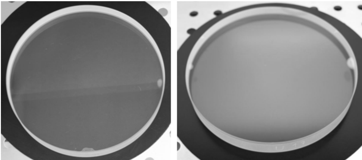
Figure 6: Glass wafer bonded to massive glass substrate of identical material (left: fused silica, right: ULE)
